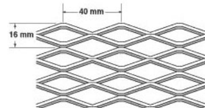
SQUARELINEmedium Dimension
