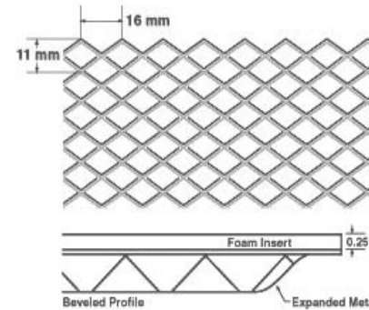
SQUARELINEstandard Dimension
